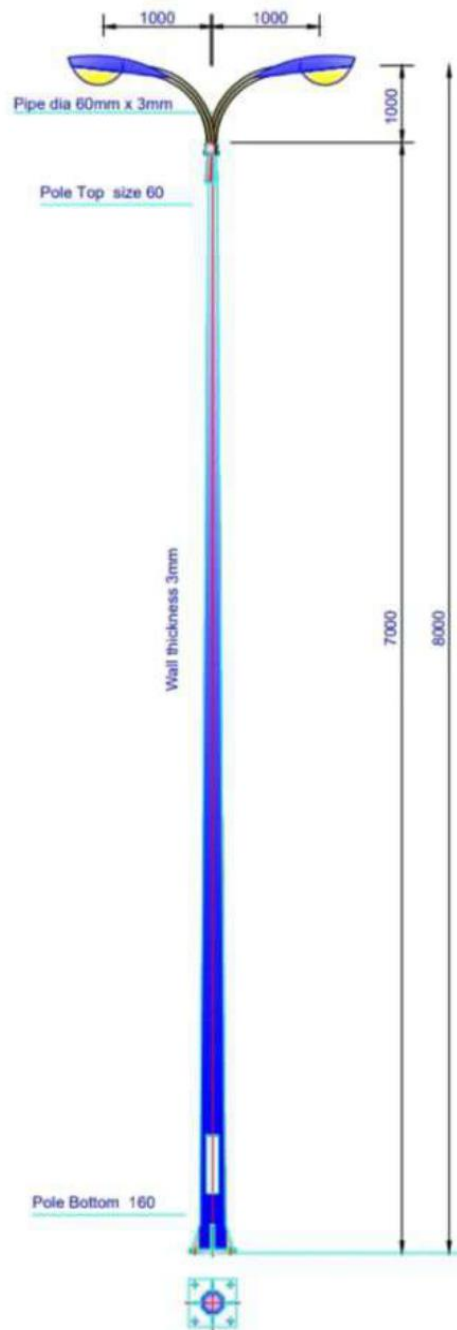
OCTAGON POLE 8 mtrs. Double ARM
